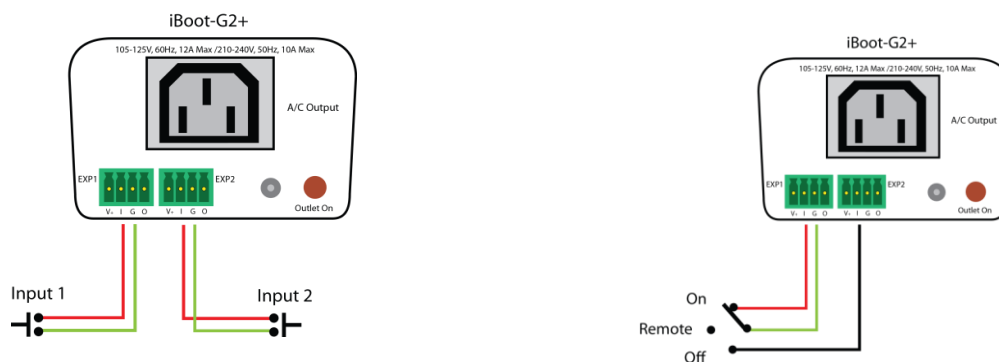
Input Connections to Switches for Power Control
